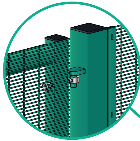
Hinge Detail
